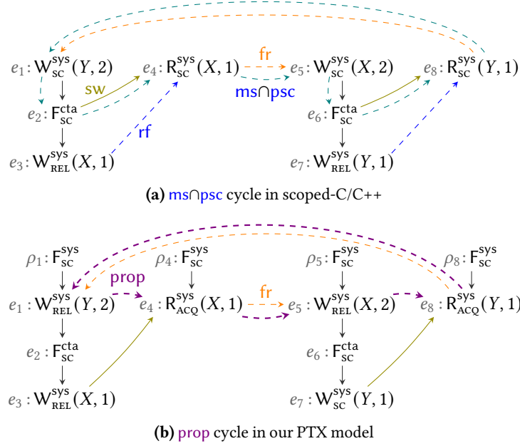
Figure 16. The execution graphs of a scoped-C/C++ program mapped to PTX. The first two threads are in a different CTA than the last two threads. Both executions are disallowed by a cycle in their respective model. Note that the sw edge to e_4 can start in either e_2 or e_3 (and to e_8 from e_6 or e_7 ) in both graphs; we draw the variant relevant for each cycle.
