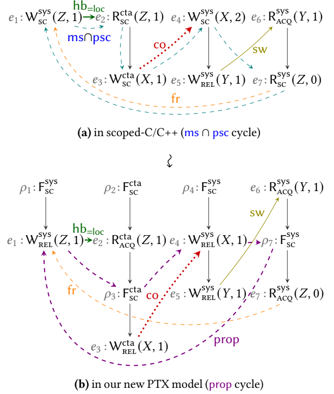
Figure 15. Execution graphs for programs in Figure 3, which maps correctly under our PTX model. The rightmost thread is in a separate CTA from the other threads.
