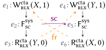
Figure 17. Store-buffering program, with threads in different CTAs. Disallowed by the pre-existing PTX model.
